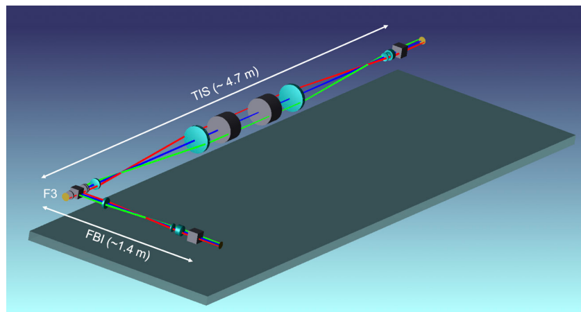
3D render of the TIS/FBI optics assembly. Credit: TIS/FBI consortium
