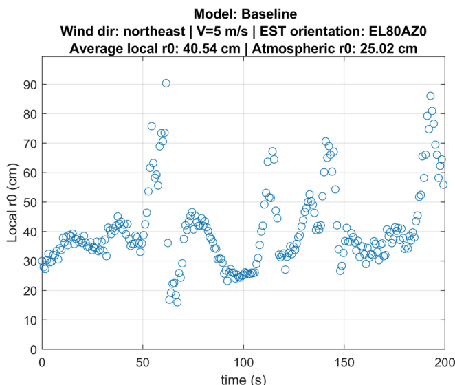
Fig. 4. Local Fried parameter during a 200 s observation.
