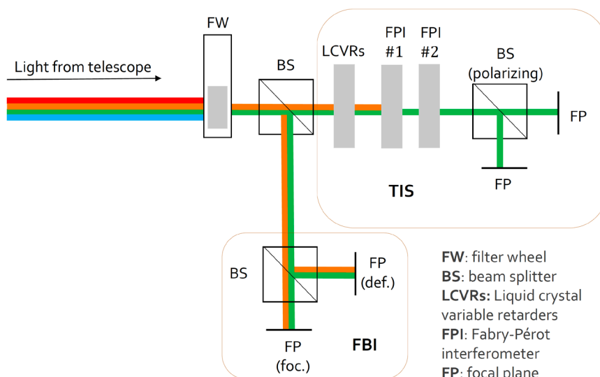
Figure 1. Conceptual layout of the TIS/FBI instrument.
